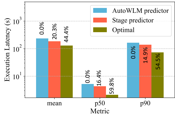
Figure 6: End-to-end performance in terms of query latency of different exec-time predictors inside Redshift. We listed the percentage improvement over the AutoWLM predictor.
