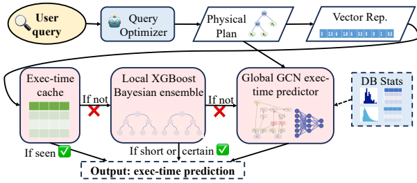
Figure 4: Workflow overview of the Stage predictor.
