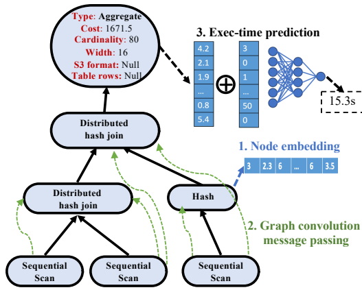
Figure 5: Global model featurization and architecture.
