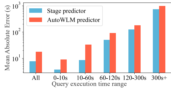
Figure 8: Prediction accuracy of stage predictor compared to the AutoWLM predictor in Redshift.
